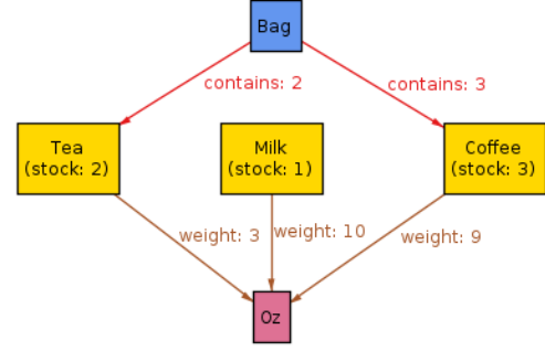
Figure 4: QALLOY counter-example to hasMilk
